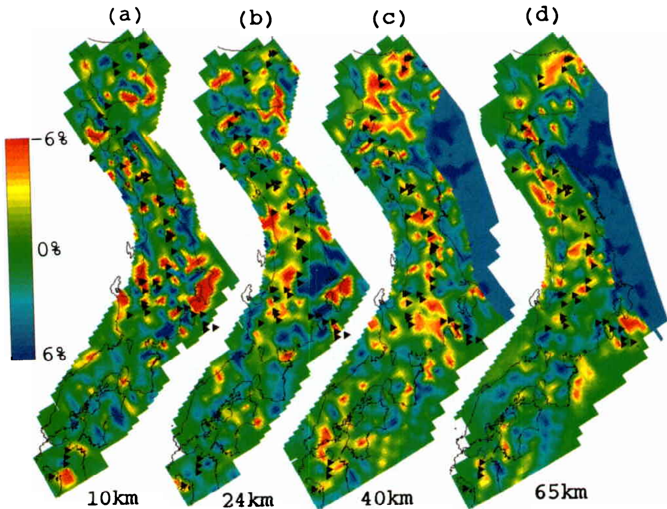
Plate 2. Fractional P wave velocity perturbations (in percent) at four depths determined by the constrained inversion (see text): (a) 10-km, (b) 24-km, (c) 40-km, (d) 65-km. Red and blue denote low and high velocities, respectively. The perturbation scale is shown on the left of the figure. Solid triangles denote active volcanoes in the Japan Islands.
