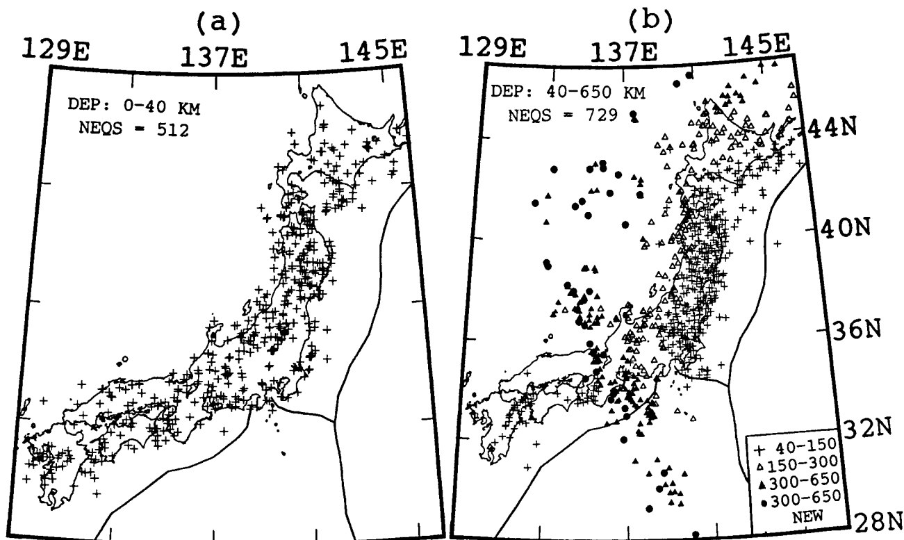
Figure 2. (a) Epicentral locations of 512 earthquakes with focal depths shallower than 40-km. (b) Epicentral locations of 729 earthquakes with focal depths from 40- to 650-km. Epicenters are shown in different symbols according to the focal depth. Cross, 40-150 km; open triangle, 150-300 km; solid triangle and solid circle, 300-650 km. Solid triangles denote deep events used by Zhao and Hasegawa [1993]; solid circles denote 41 deep earthquakes which are newly added in this study.
