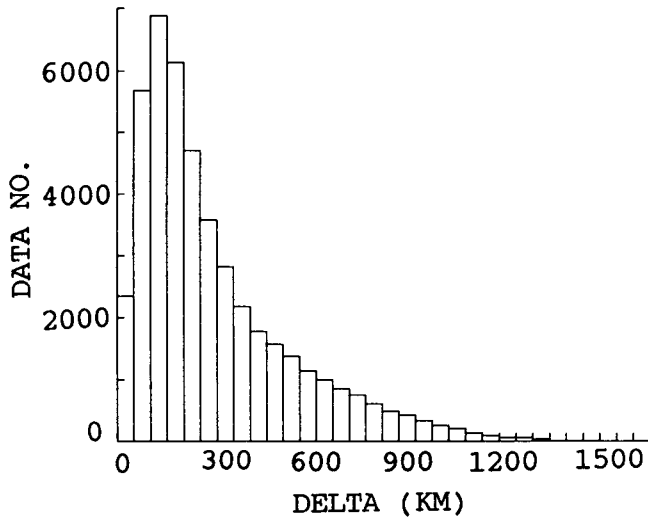
Figure 3. Number of P wave arrival times from local and regional events versus epicentral distances.
